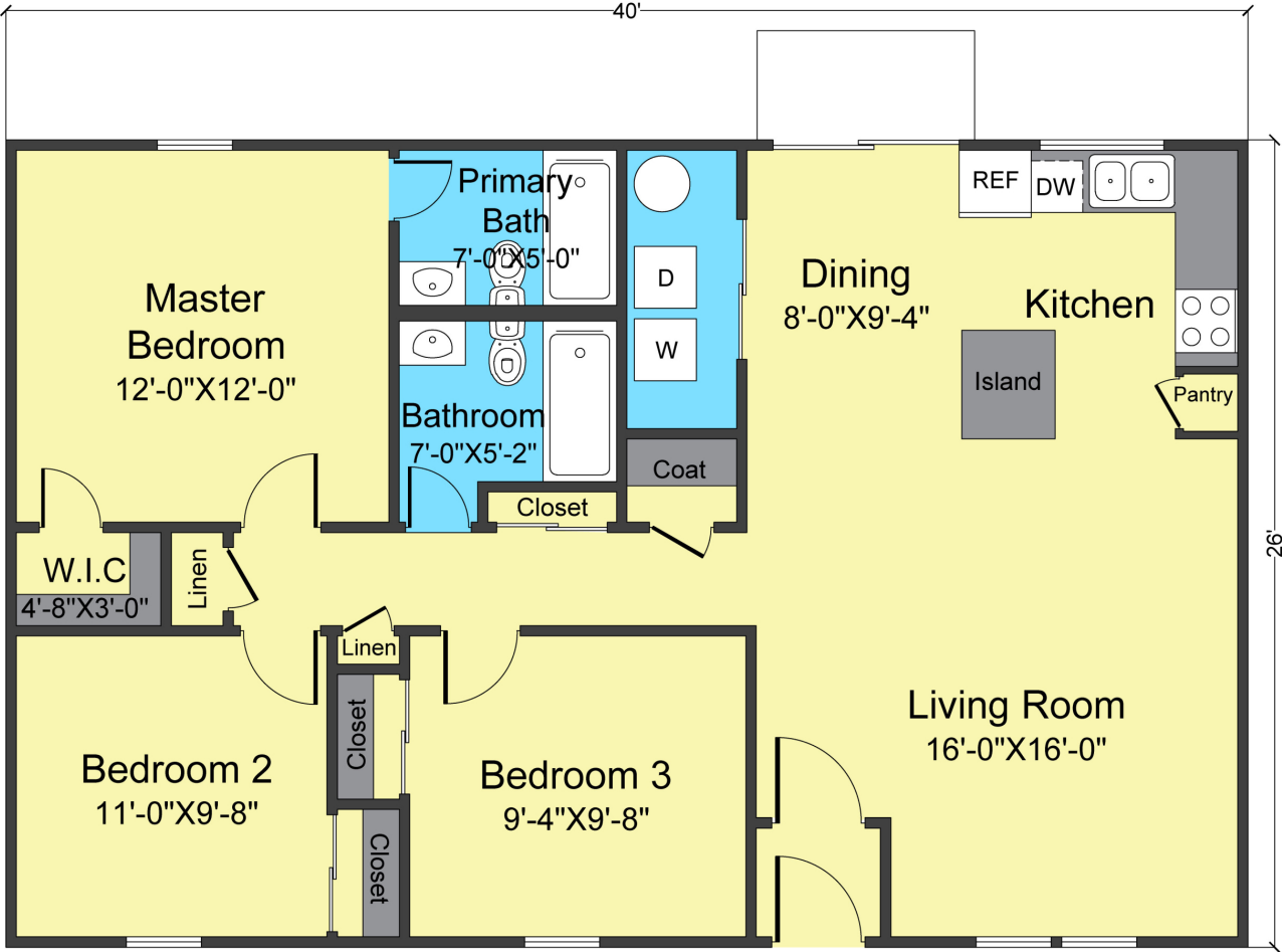
Floor Plan
