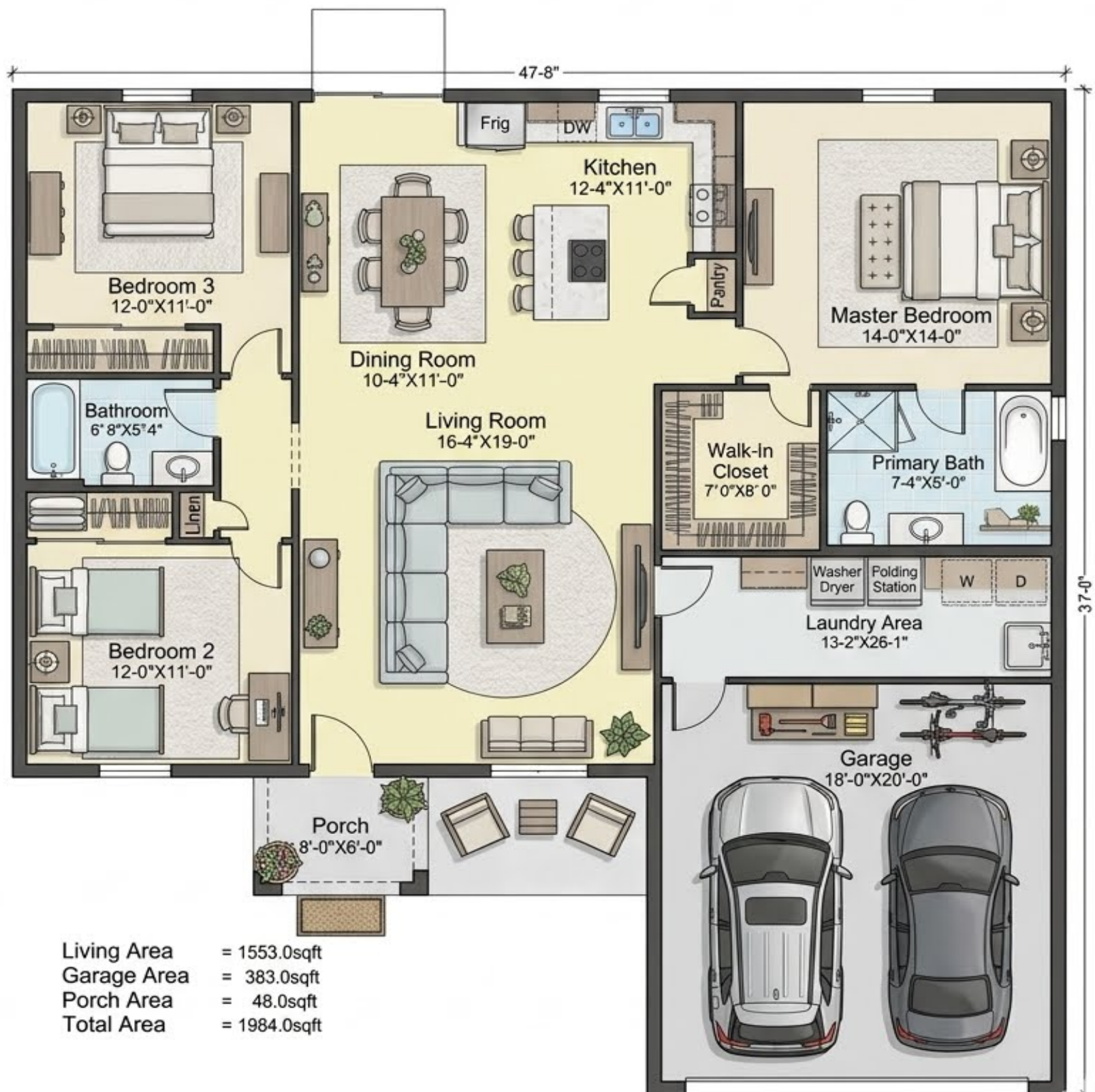
Floor Plan
