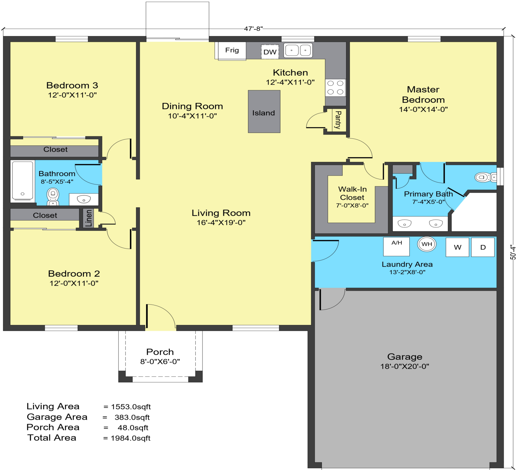
Floor Plan
