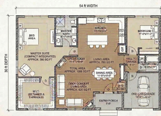
SINGLE STORY RESIDENCE FLOOR PLAN - EXPANDED MASTER SUITE WITH GARAGE
