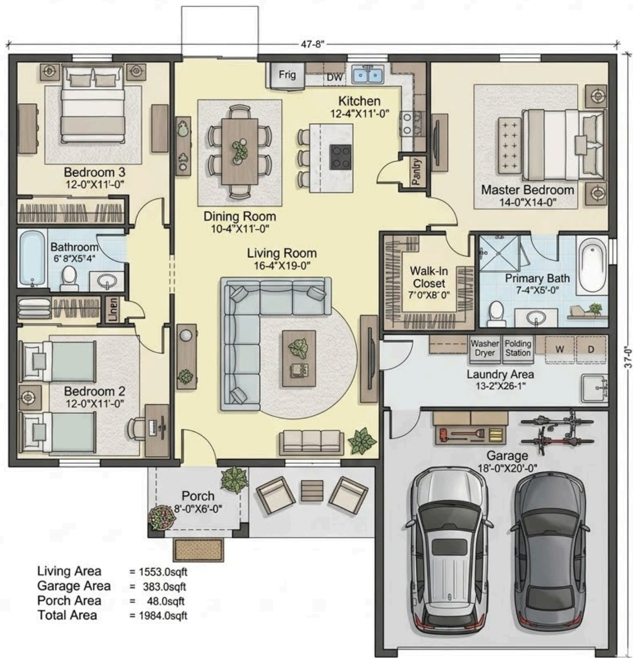
Floor Plan
