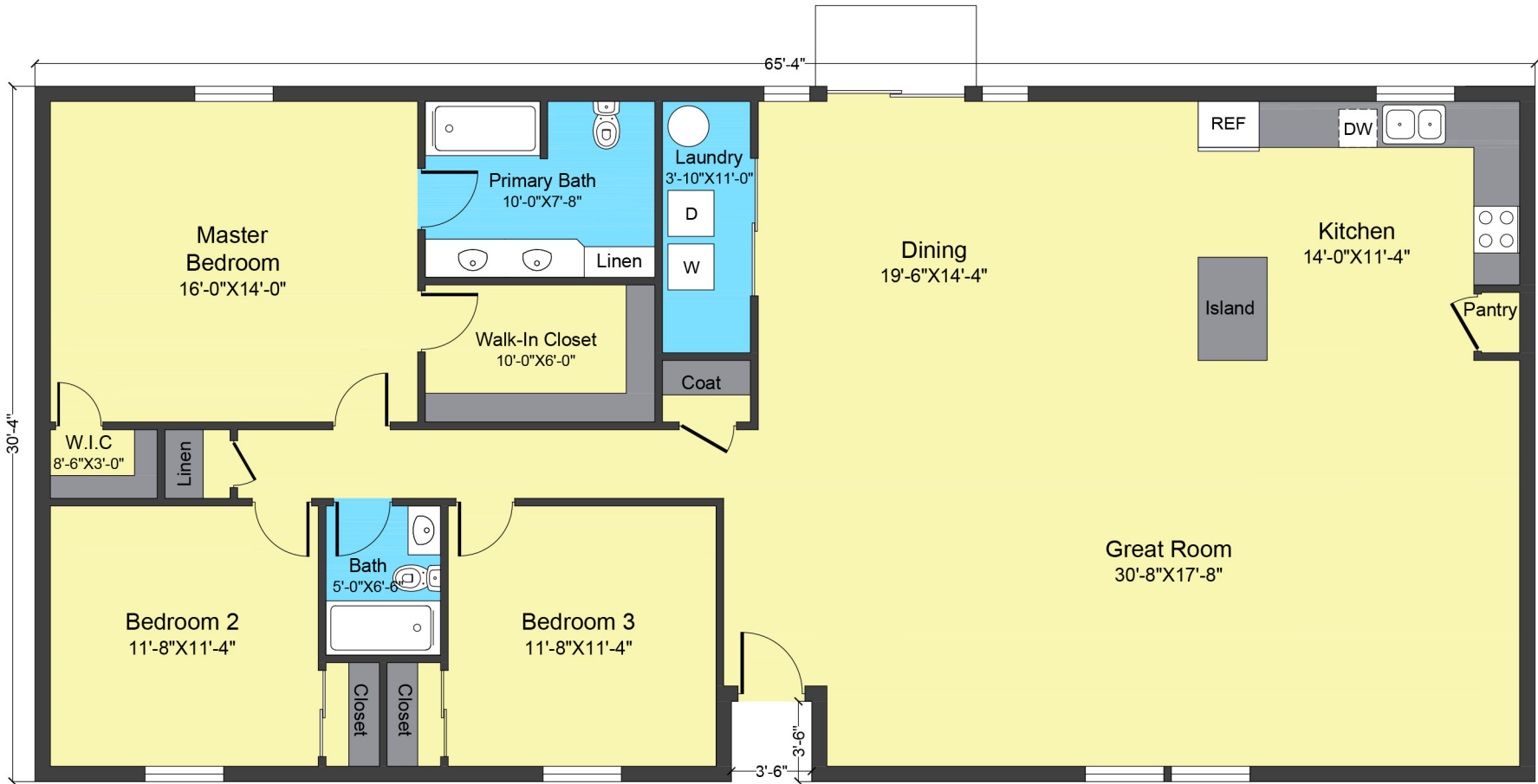
Floor Plan
